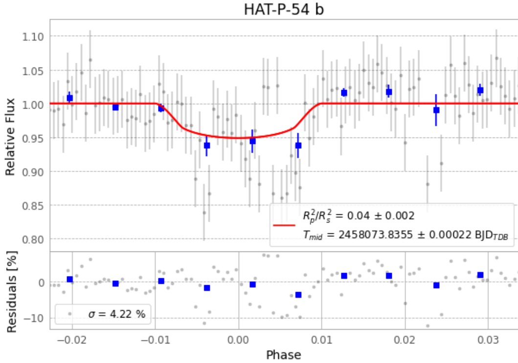
Figure 1 — FinalLightCurve_HAT-P-54 b_2017-11-15.png (SHA-256 dd3bb7dab9e9eb43...)
