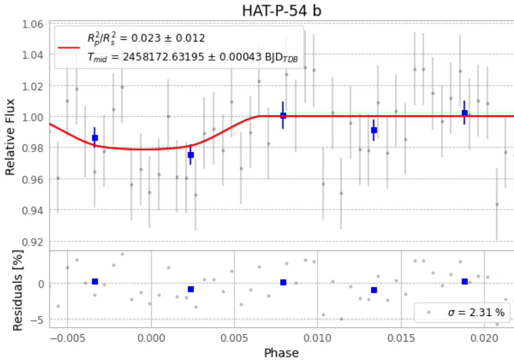
Figure 1 — FinalLightCurve_HAT-P-54 b_2018-02-22.png (SHA-256 70481c92273f5e52...)
