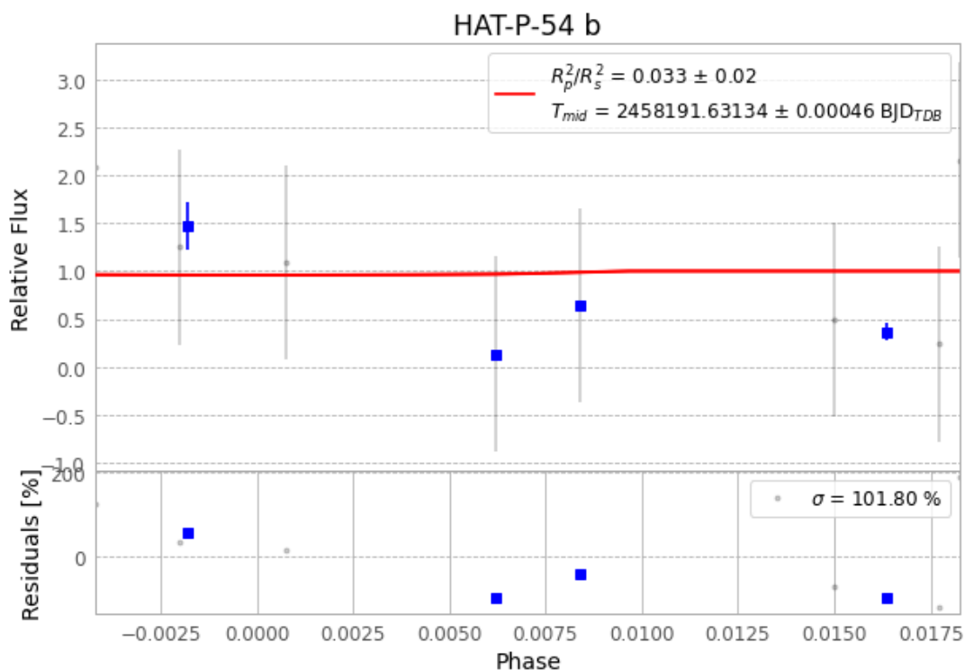
Figure 1 — FinalLightCurve_HAT-P-54 b_2018-03-13.png (SHA-256 a04c8b7ca6430b60...)
