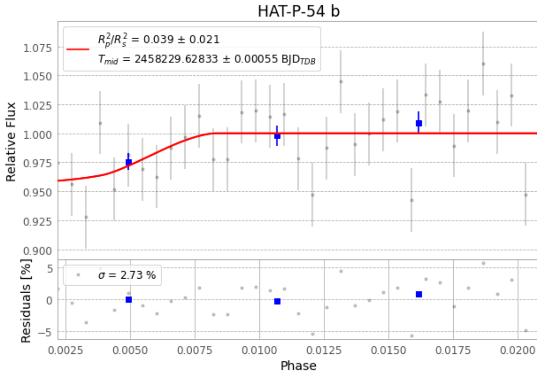
Figure 1 — FinalLightCurve_HAT-P-54 b_2018-04-20.png (SHA-256 a8598a1b247e7ddd...)
