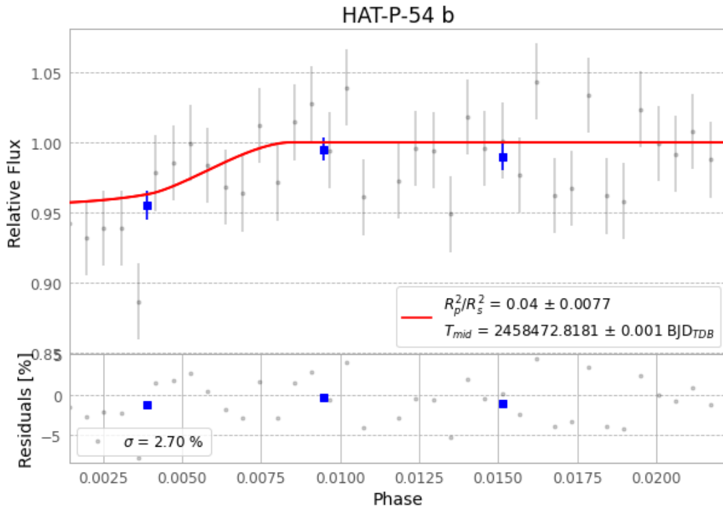
Figure 1 — FinalLightCurve_HAT-P-54 b_2018-12-20.png (SHA-256 50a399542ef8175e...)
