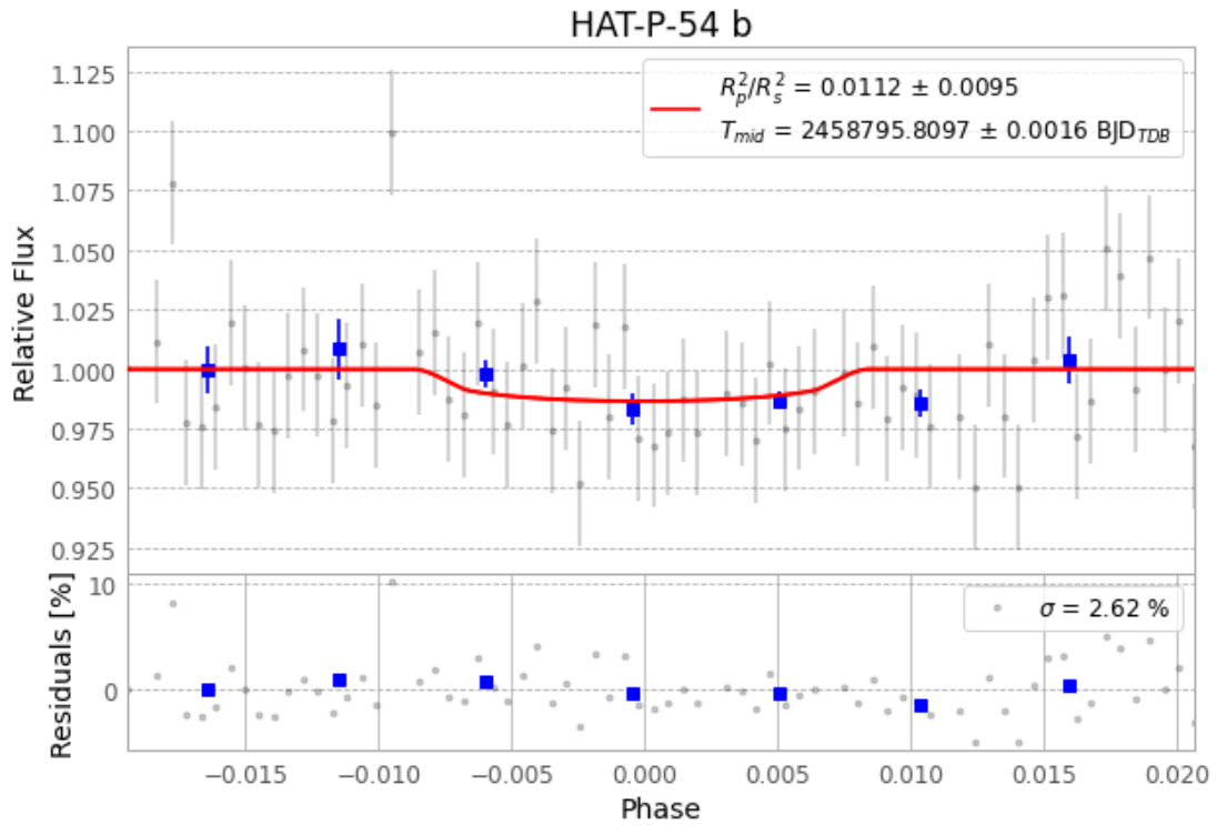
Figure 1 — FinalLightCurve_HAT-P-54 b_2019-11-07.png (SHA-256 752d88adc7203657...)
