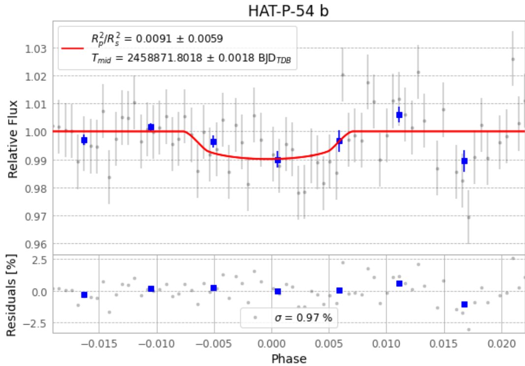
Figure 1 — FinalLightCurve_HAT-P-54 b_2020-01-22.png (SHA-256 e1a7b3ea5524f55c...)
