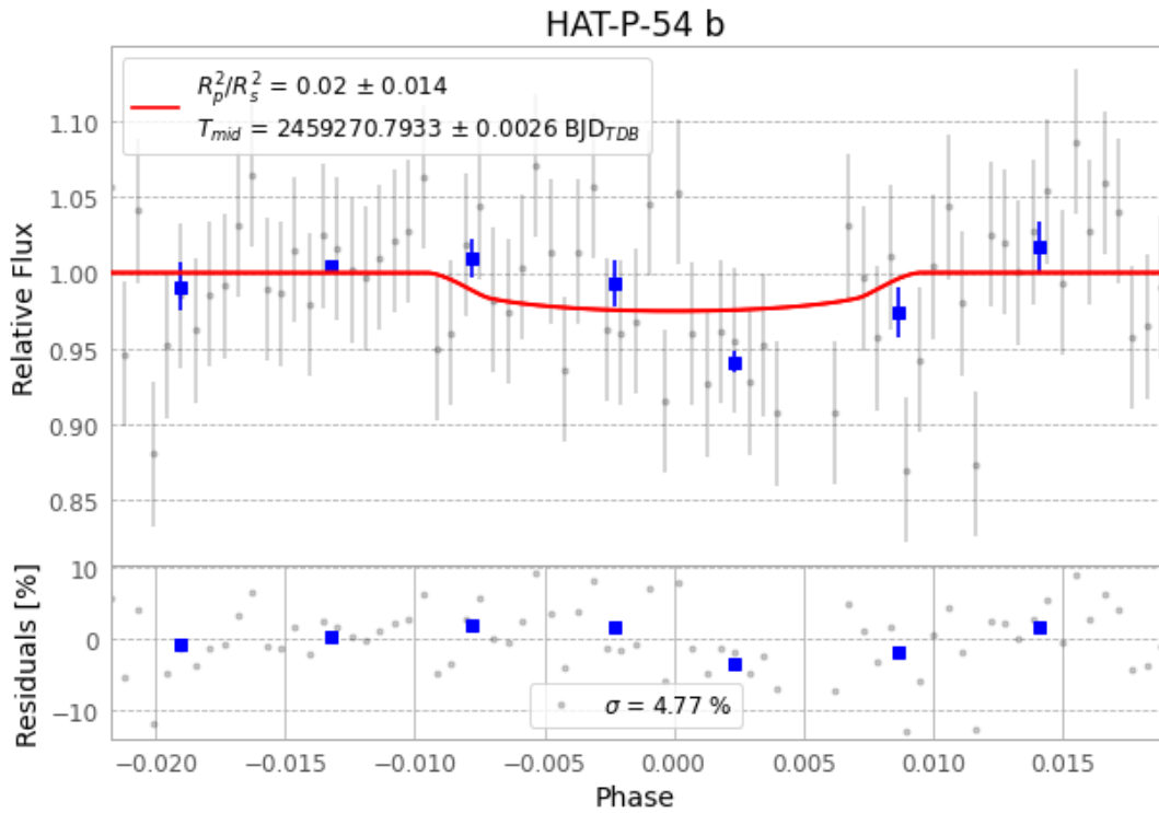
Figure 1 — FinalLightCurve_HAT-P-54 b_2021-02-24.png (SHA-256 c929551976aefc2d...)
