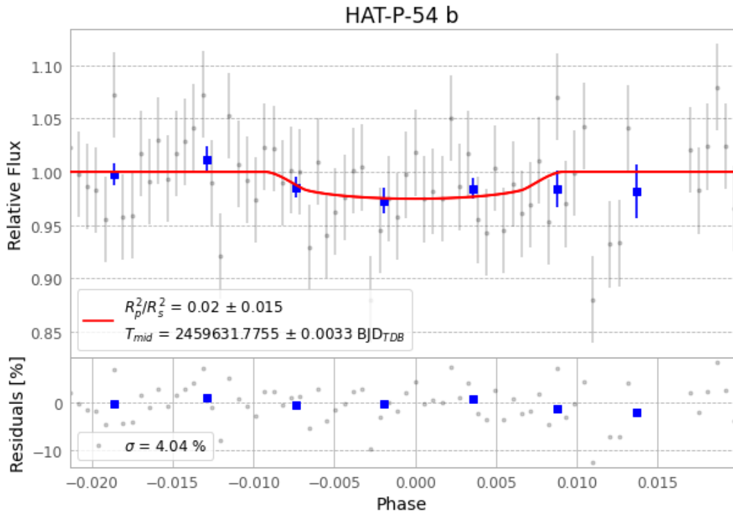
Figure 1 — FinalLightCurve_HAT-P-54 b_2022-02-20.png (SHA-256 9c4334797c1020f4...)
