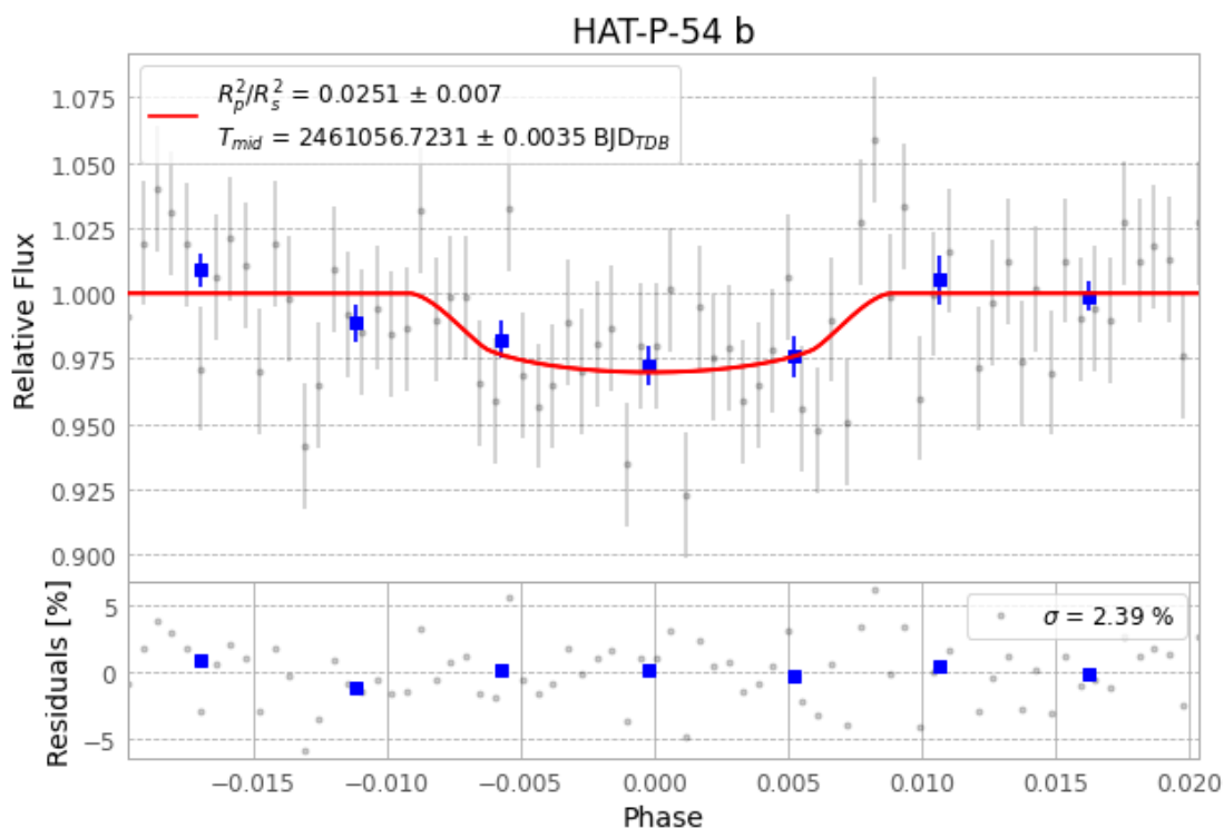
Figure 1 — FinalLightCurve_HAT-P-54 b_2026-01-15.png (SHA-256 a1d2ca97d54af6f6...)
