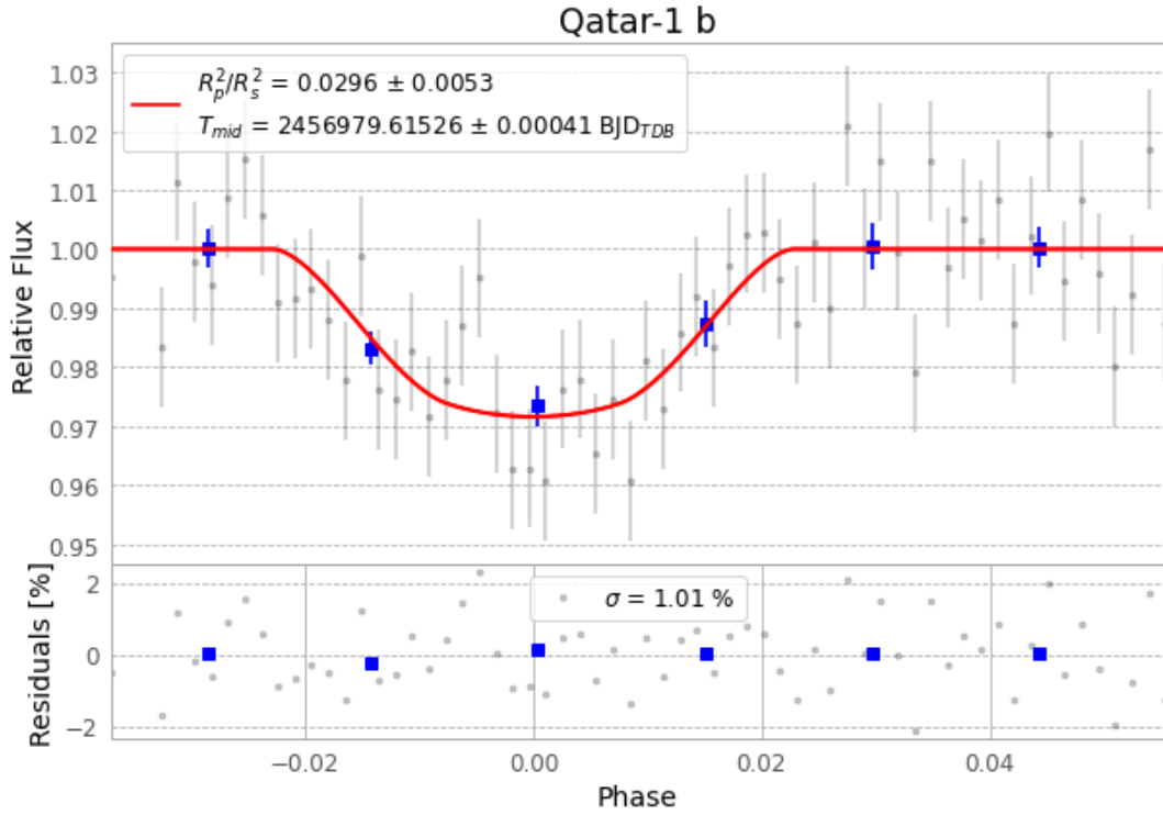
Figure 1 — FinalLightCurve_Qatar-1 b_2014-11-17.png (SHA-256 3ff3421d4a7e2515...)
