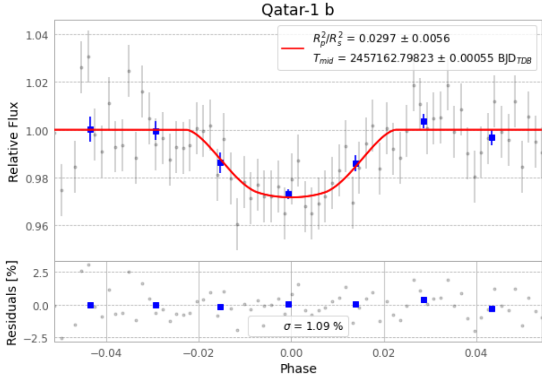
Figure 1 — FinalLightCurve_Qatar-1 b_2015-05-19.png (SHA-256 c8dff56b7f0d70b7...)
