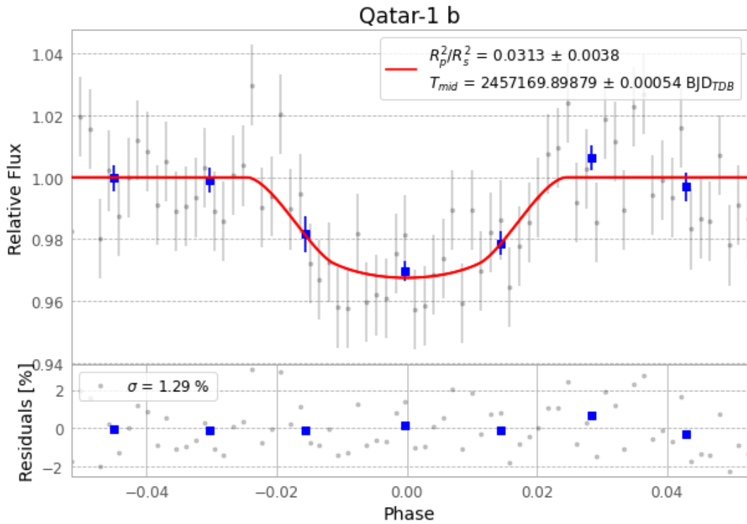
Figure 1 — FinalLightCurve_Qatar-1 b_2015-05-27.png (SHA-256 d1fd983c03761c76...)
