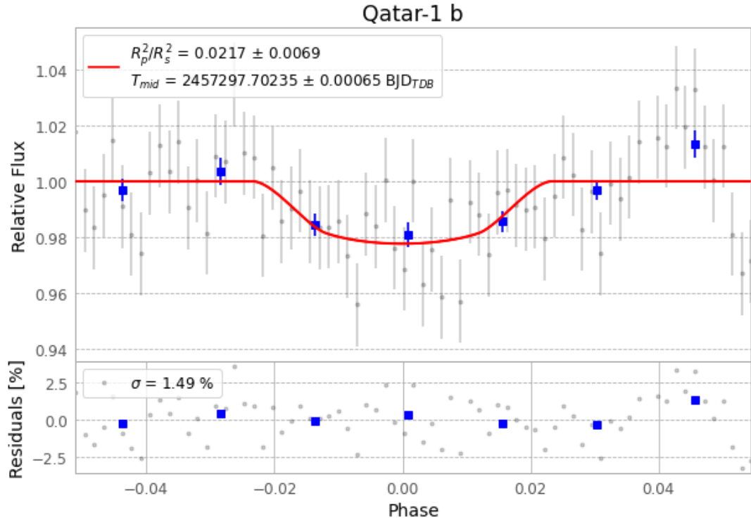
Figure 1 — FinalLightCurve_Qatar-1 b_2015-10-01.png (SHA-256 93ec95d422acaa72...)
