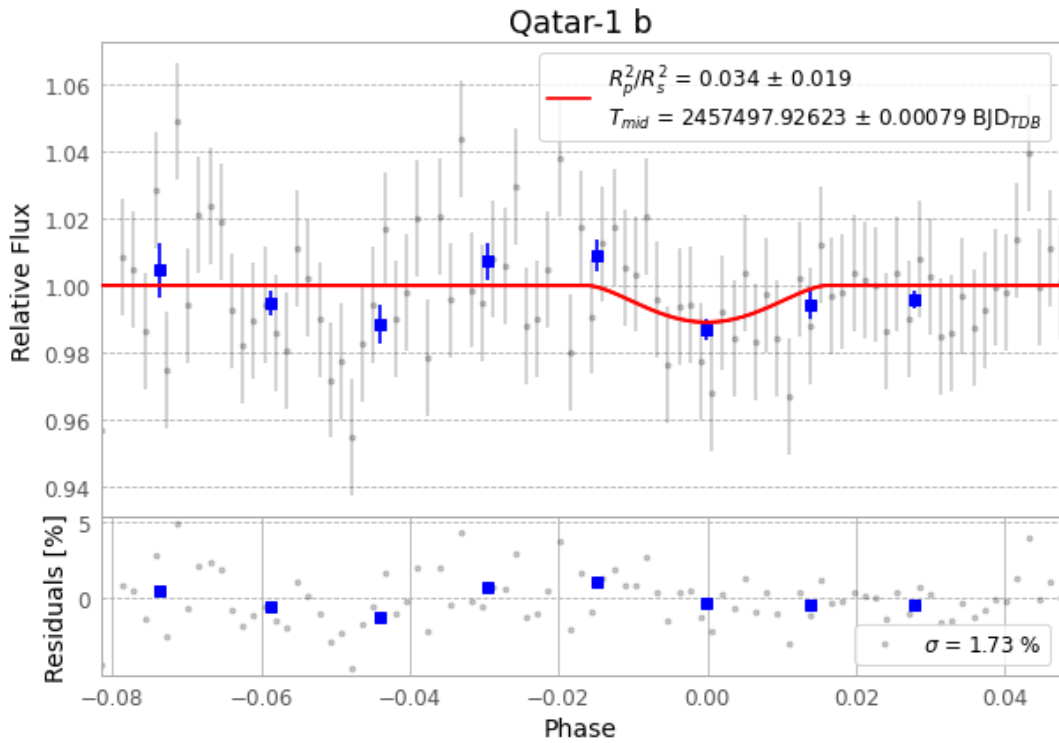
Figure 1 — FinalLightCurve_Qatar-1 b_2016-04-19.png (SHA-256 b0e0e48b7d4836d6...)
