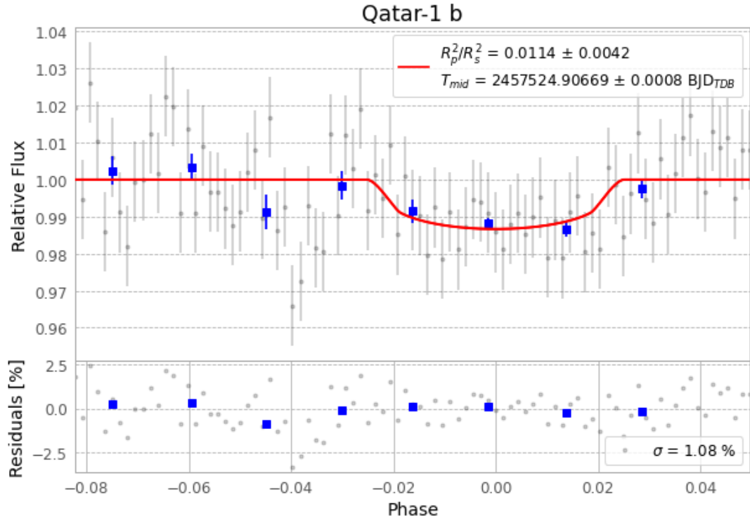
Figure 1 — FinalLightCurve_Qatar-1 b_2016-05-15.png (SHA-256 02fd95ca0af6475e...)
