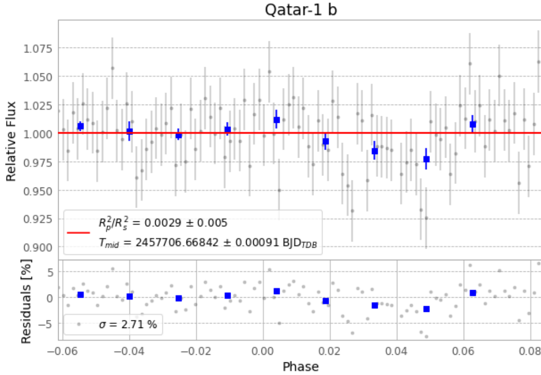
Figure 1 — FinalLightCurve_Qatar-1 b_2016-11-13.png (SHA-256 922a54d2c304aba2...)
