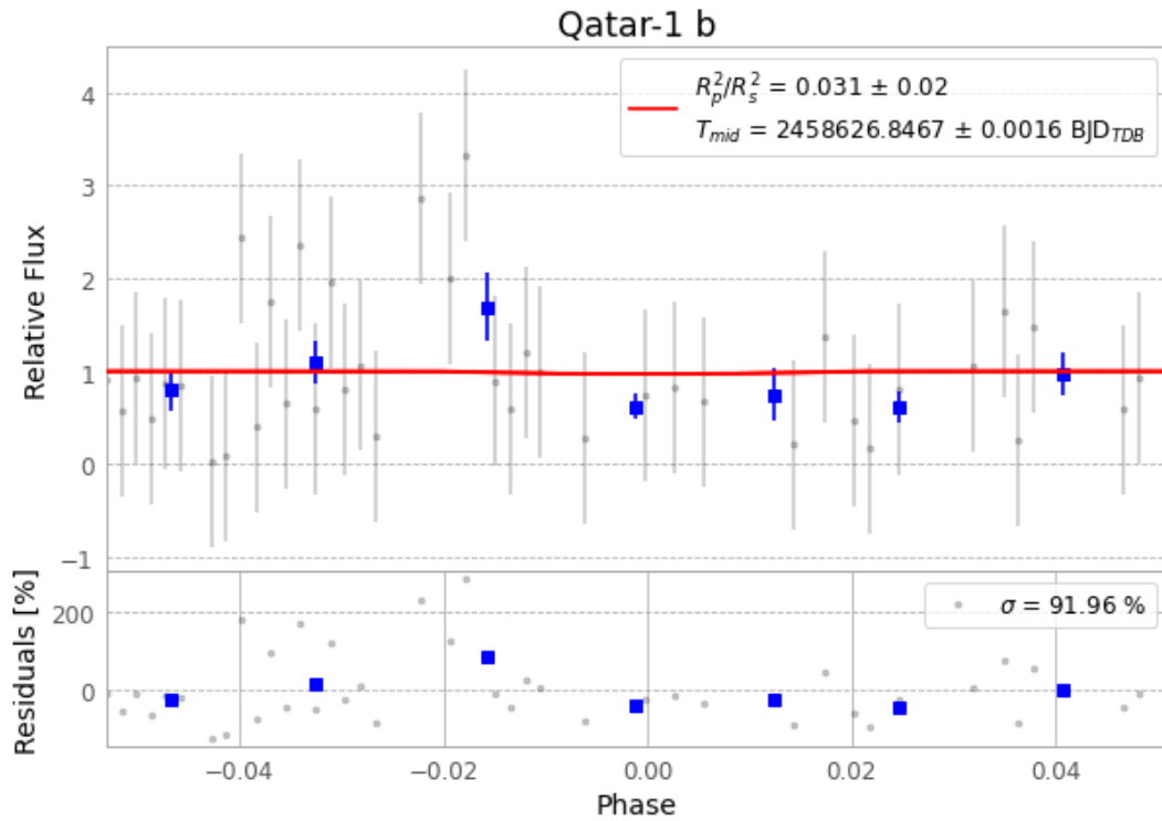
Figure 1 — FinalLightCurve_Qatar-1 b_2019-05-22.png (SHA-256 5dc32564103f1656...)
