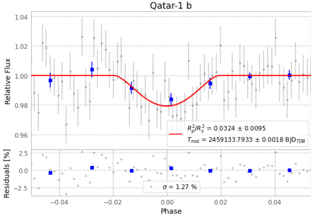
Figure 1 — FinalLightCurve_Qatar-1 b_2020-10-10.png (SHA-256 24c95ecb481a2b7e...)
