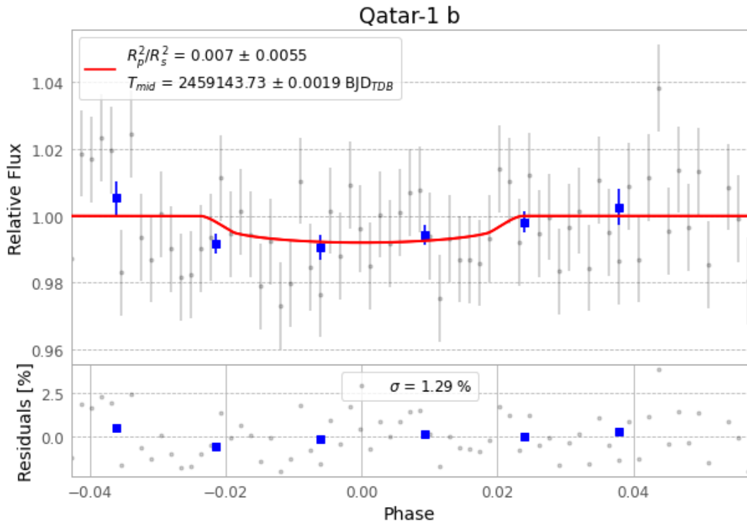
Figure 1 — FinalLightCurve_Qatar-1 b_2020-10-20.png (SHA-256 27798c4f4dbb963c...)
