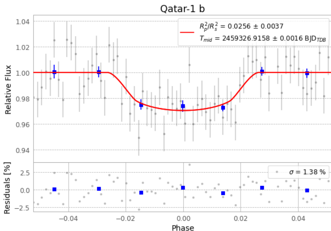
Figure 1 — FinalLightCurve_Qatar-1 b_2021-04-22.png (SHA-256 47819674c3705005...)
