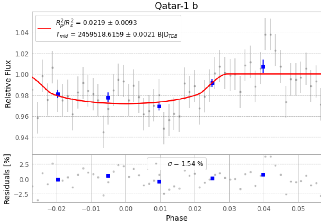
Figure 1 — FinalLightCurve_Qatar-1 b_2021-10-30.png (SHA-256 dd56145cd1480cda...)
