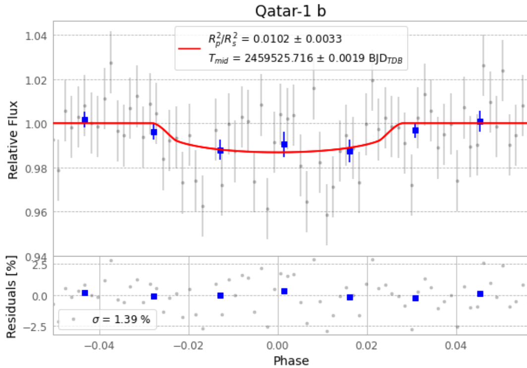
Figure 1 — FinalLightCurve_Qatar-1 b_2021-11-06.png (SHA-256 40a4b0744633a278...)
