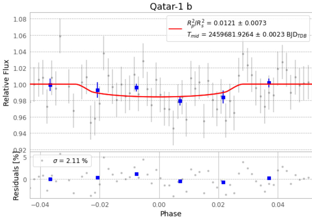
Figure 1 — FinalLightCurve_Qatar-1 b_2022-04-12.png (SHA-256 1cd1e8ac7aaaa680...)
