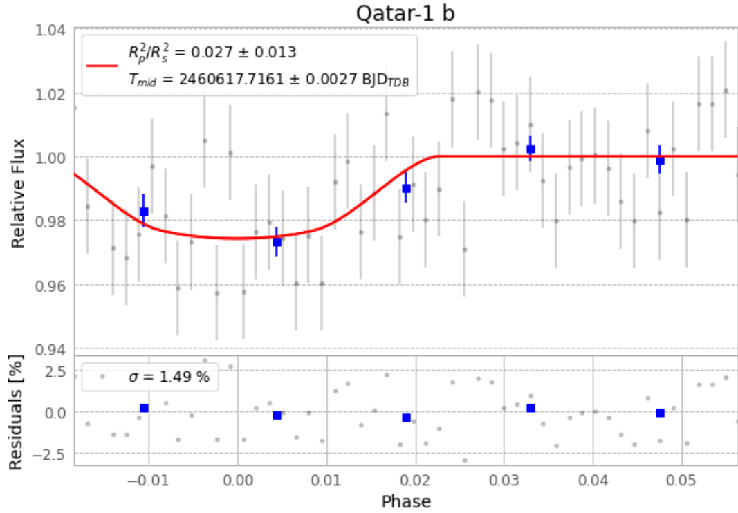
Figure 1 — FinalLightCurve_Qatar-1 b_2024-11-02.png (SHA-256 160d4201b65f573c...)
