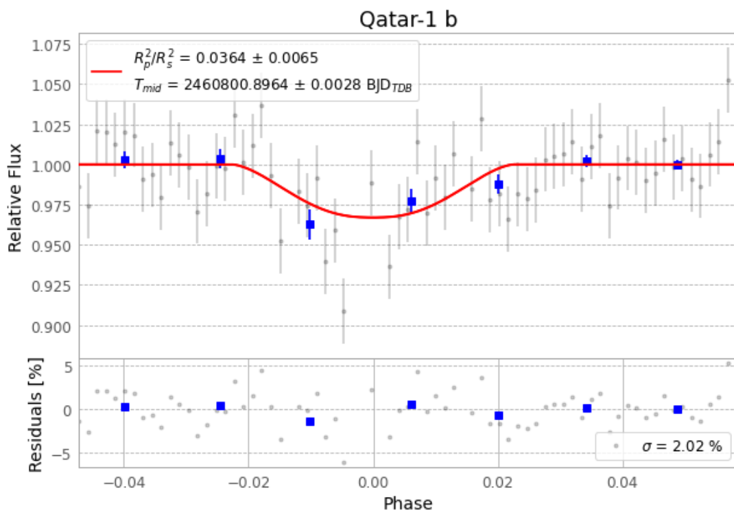
Figure 1 — FinalLightCurve_Qatar-1 b_2025-05-05.png (SHA-256 cde3865f47c94a98...)
