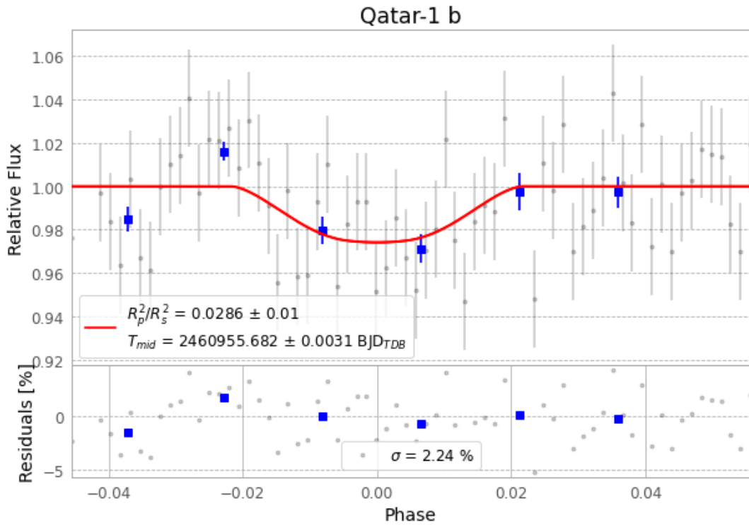
Figure 1 — FinalLightCurve_Qatar-1 b_2025-10-06.png (SHA-256 0124efcdf158a4ca...)
