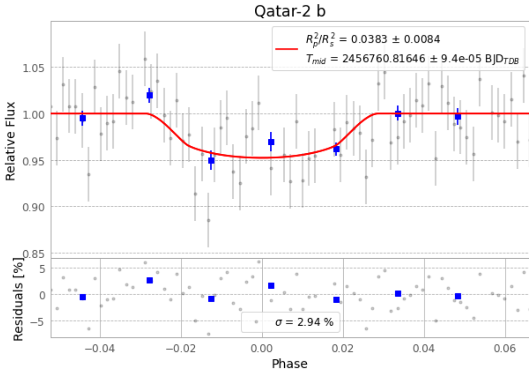
Figure 1 — FinalLightCurve_Qatar-2 b_2014-04-12.png (SHA-256 7dd2026447931262...)
