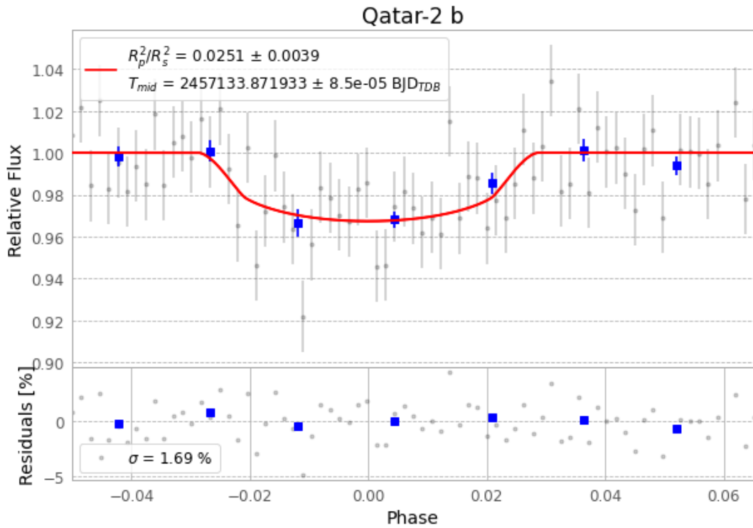
Figure 1 — FinalLightCurve_Qatar-2 b_2015-04-21.png (SHA-256 4af9ade57978b1e3...)
