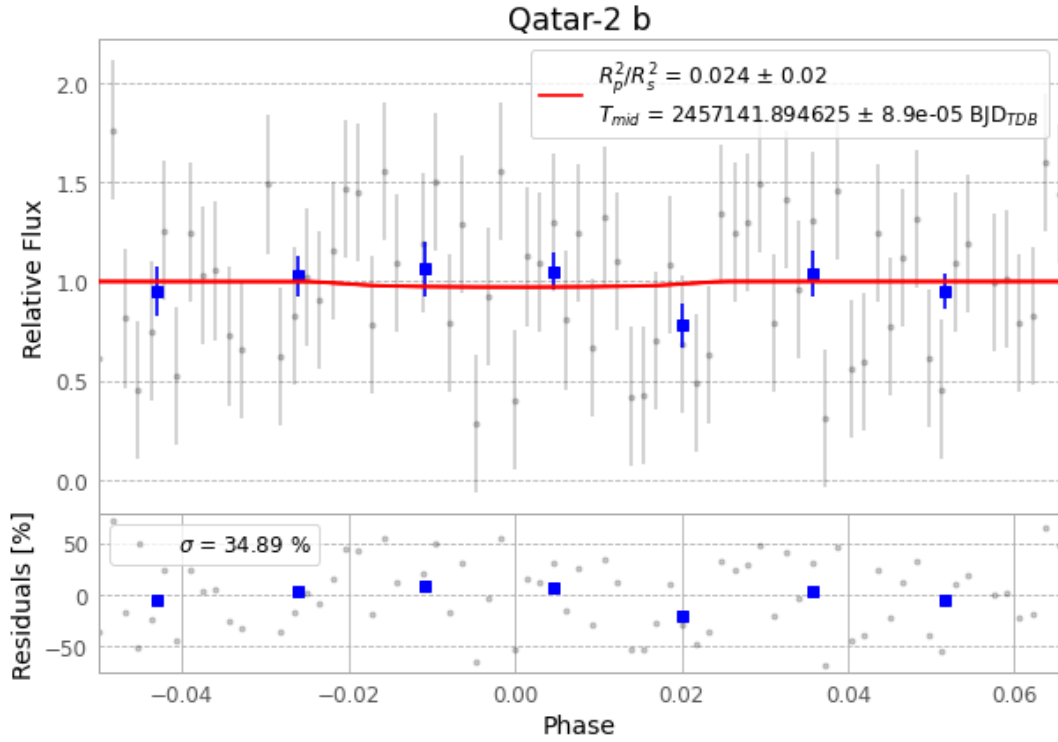
Figure 1 — FinalLightCurve_Qatar-2 b_2015-04-29.png (SHA-256 bf309bb208d5d9ad...)
