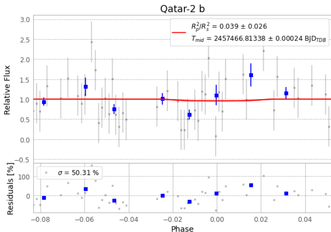
Figure 1 — FinalLightCurve_Qatar-2 b_2016-03-18.png (SHA-256 78faf25ed1579fc6...)
