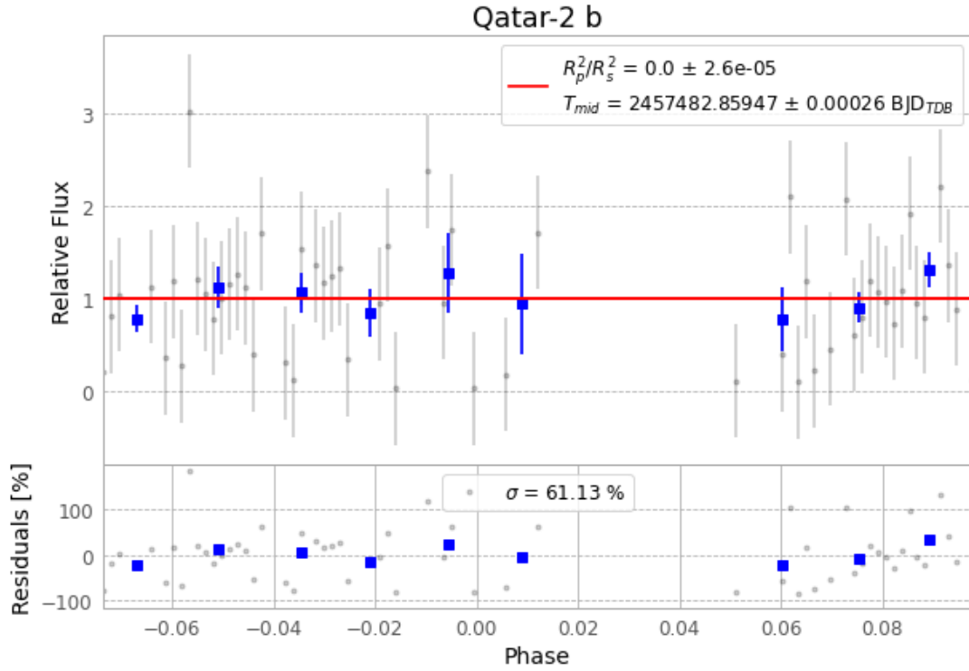
Figure 1 — FinalLightCurve_Qatar-2 b_2016-04-03.png (SHA-256 2961e6db57115408...)
