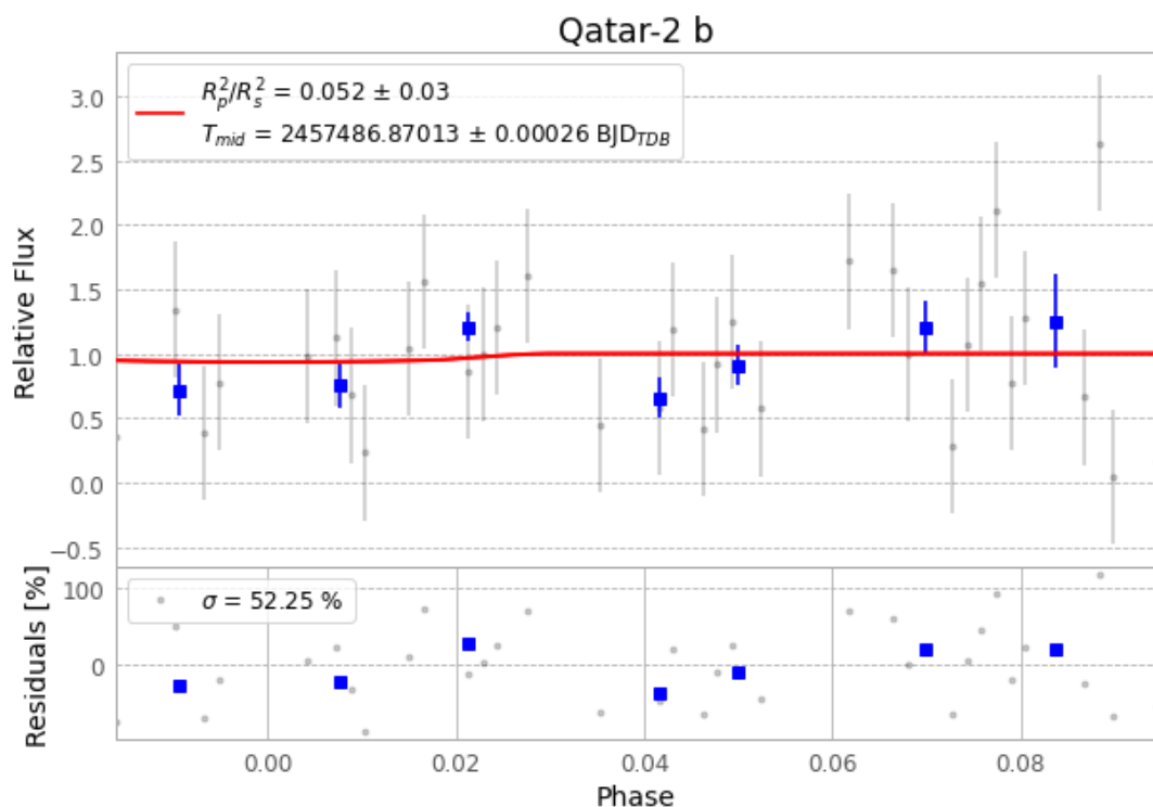
Figure 1 — FinalLightCurve_Qatar-2 b_2016-04-08.png (SHA-256 3f9f849516213be9...)
