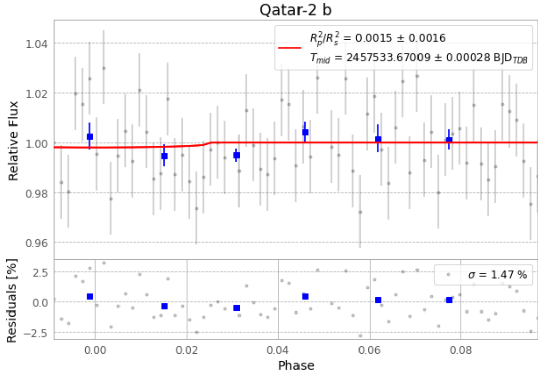
Figure 1 — FinalLightCurve_Qatar-2 b_2016-05-24.png (SHA-256 382ef6da030925c7...)
