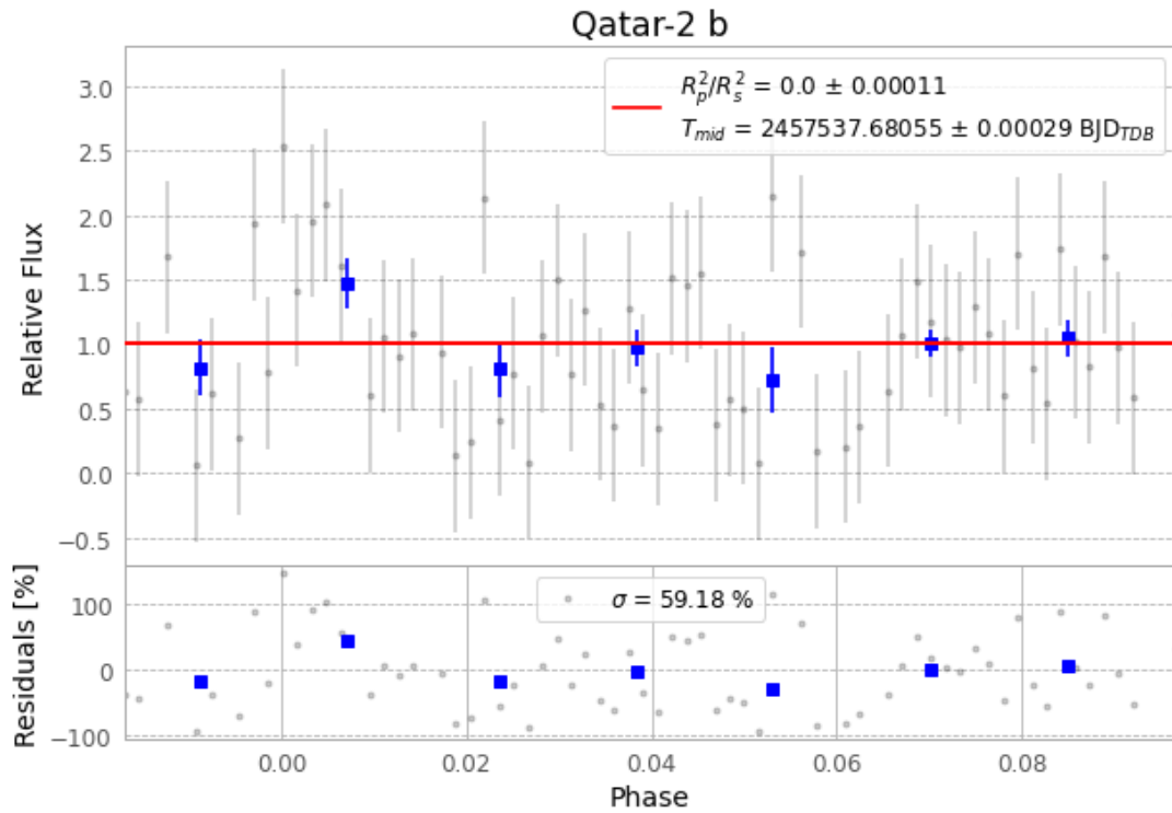
Figure 1 — FinalLightCurve_Qatar-2 b_2016-05-28.png (SHA-256 9045612f5a091fbb...)
