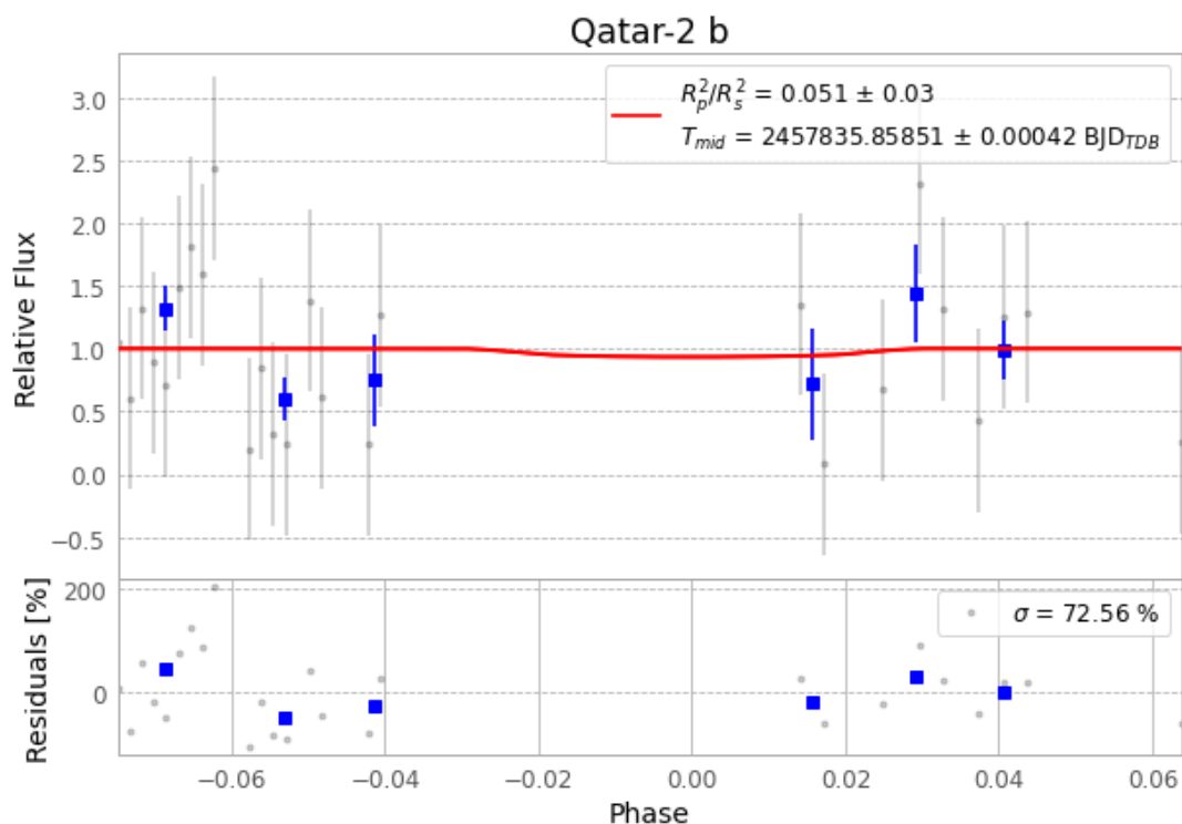
Figure 1 — FinalLightCurve_Qatar-2 b_2017-03-22.png (SHA-256 e1eab6b11717fd35...)
