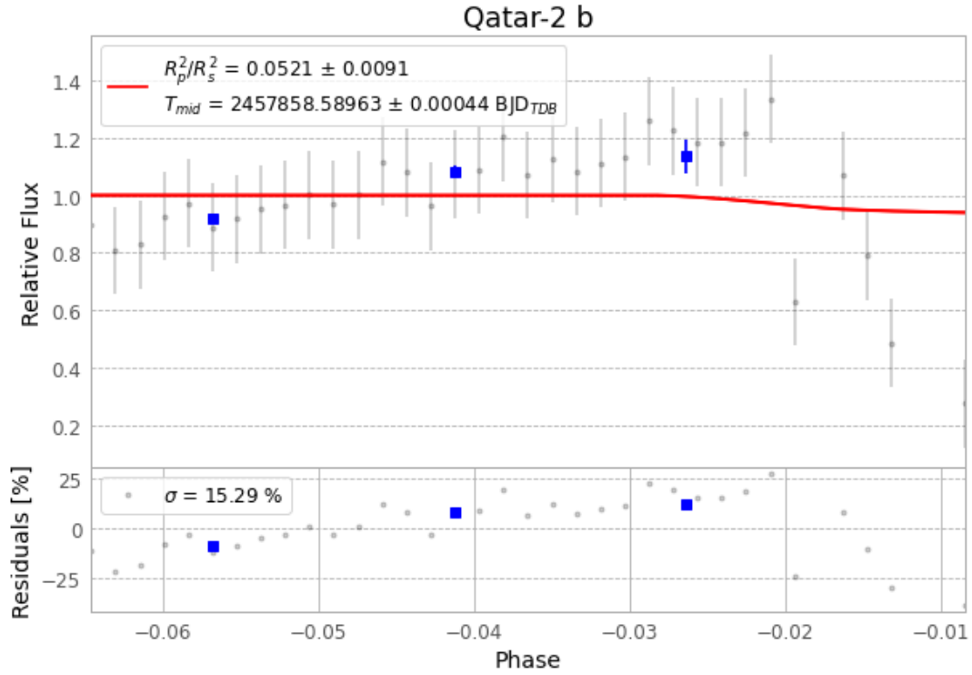
Figure 1 — FinalLightCurve_Qatar-2 b_2017-04-16.png (SHA-256 41934197636e0008...)
