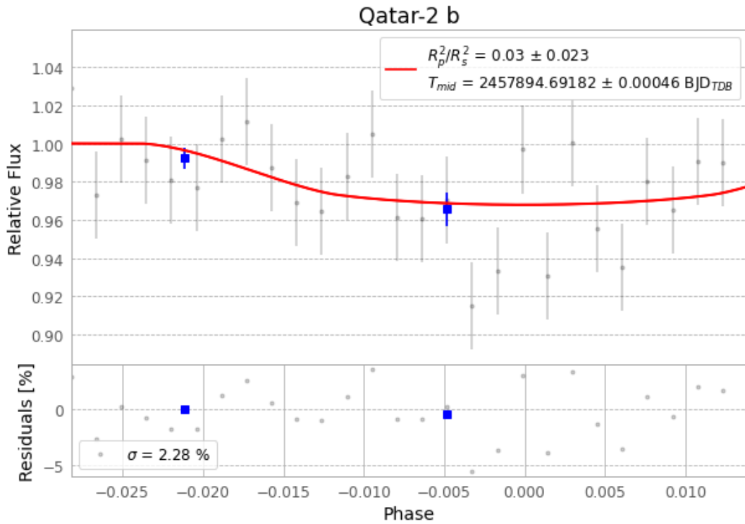
Figure 1 — FinalLightCurve_Qatar-2 b_2017-05-20.png (SHA-256 93a9fe392f6fed92...)
