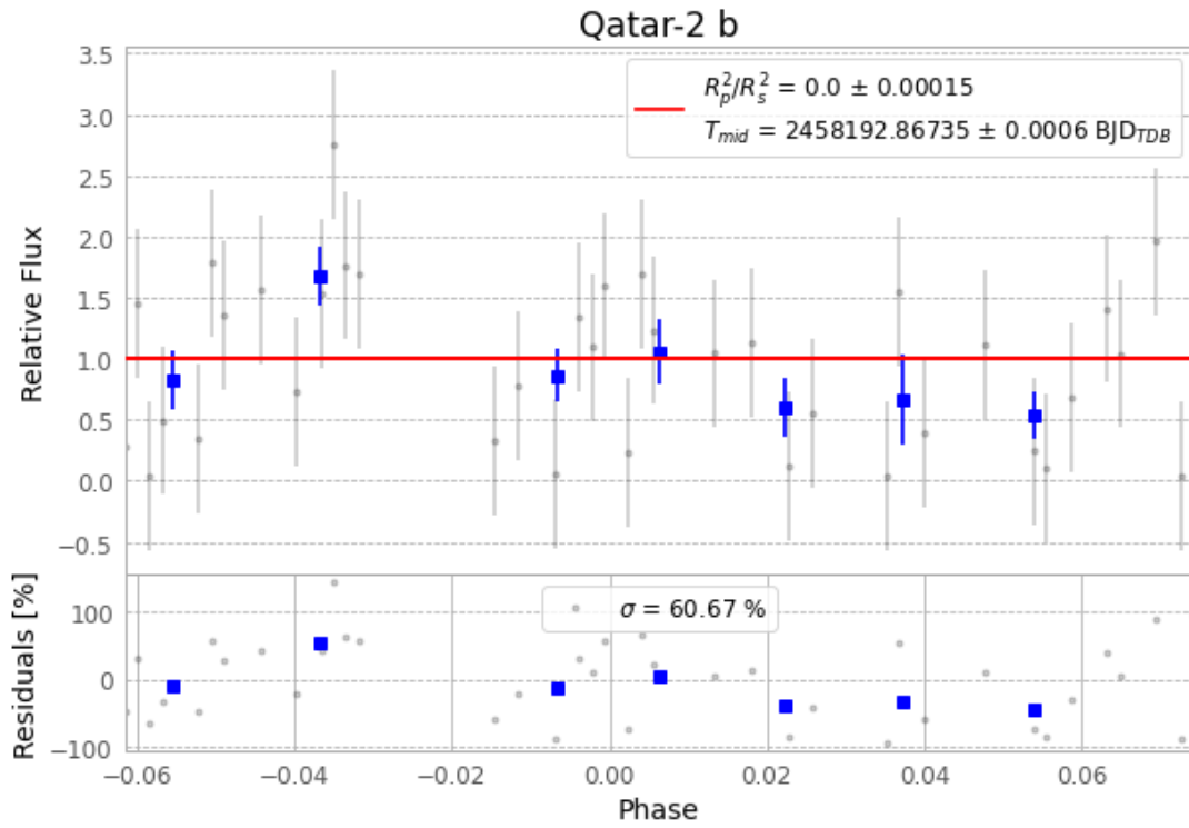
Figure 1 — FinalLightCurve_Qatar-2 b_2018-03-14.png (SHA-256 84f451a5ebbec6fb...)
