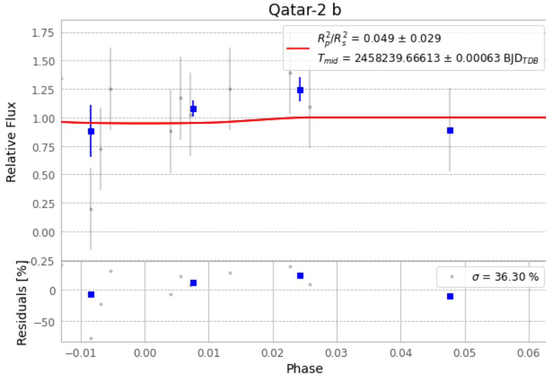
Figure 1 — FinalLightCurve_Qatar-2 b_2018-04-30.png (SHA-256 45a21a15b22e7c6c...)
