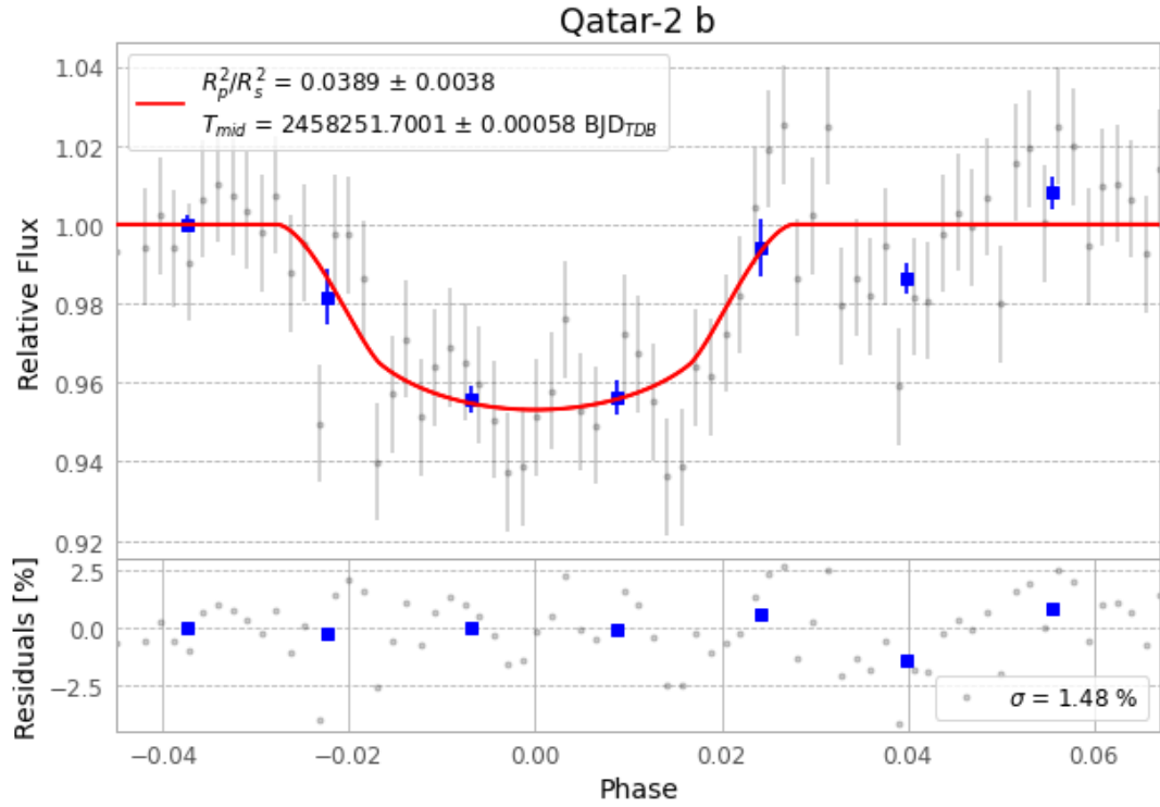
Figure 1 — FinalLightCurve_Qatar-2 b_2018-05-12.png (SHA-256 9fa2dec13c39273e...)
