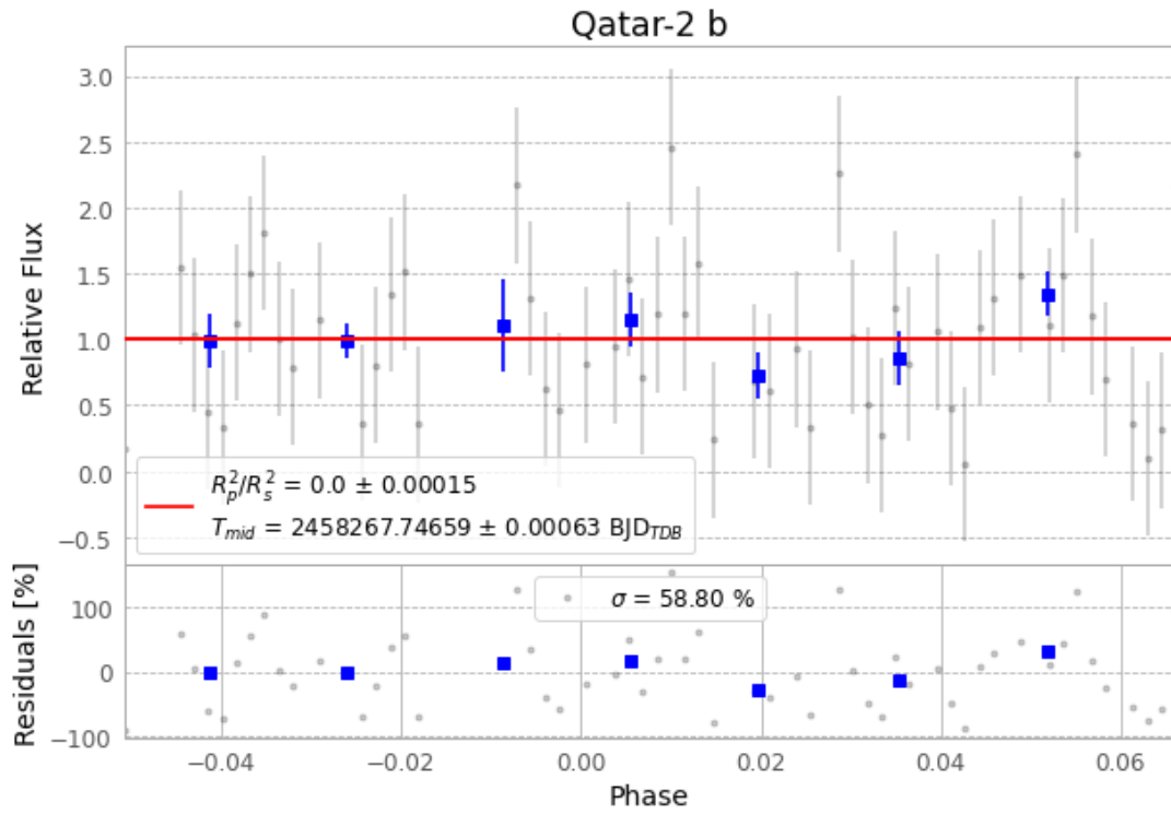
Figure 1 — FinalLightCurve_Qatar-2 b_2018-05-28.png (SHA-256 372f3fa4fbe91b71...)
