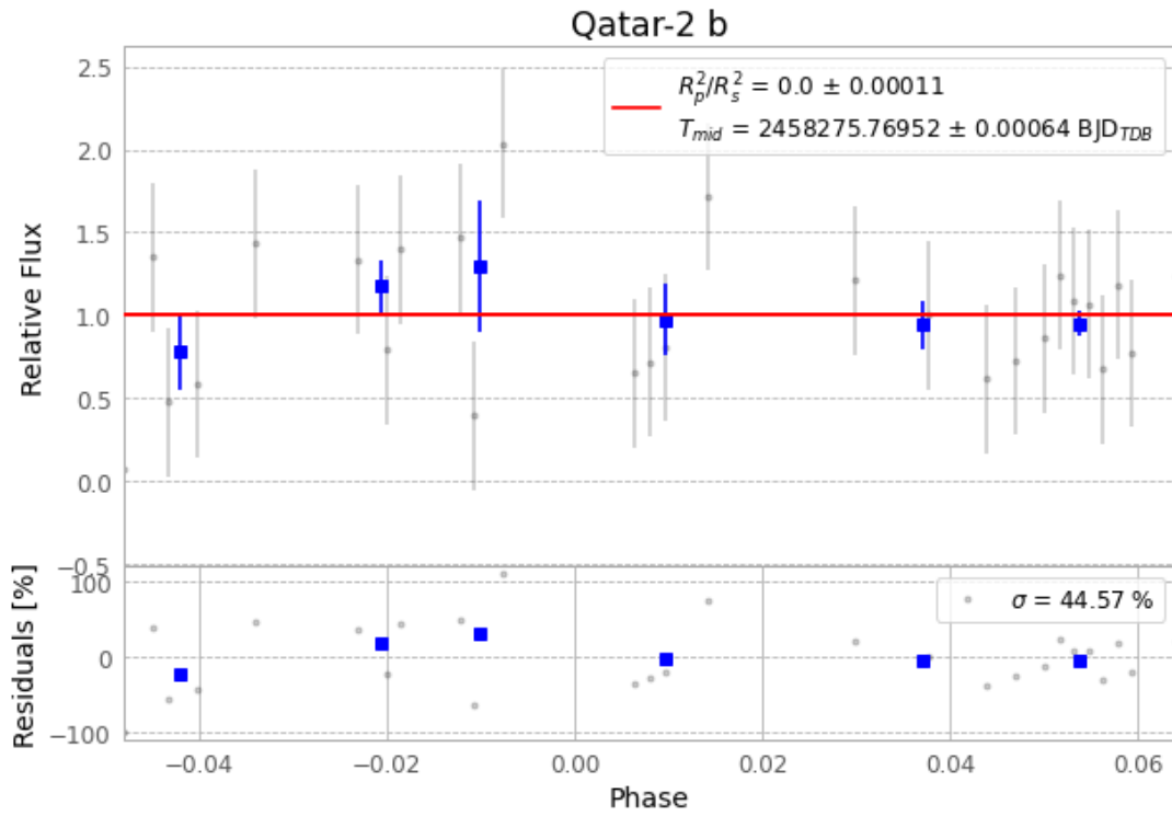
Figure 1 — FinalLightCurve_Qatar-2 b_2018-06-05.png (SHA-256 3d228a6f118fc36d...)
