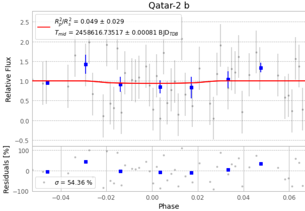
Figure 1 — FinalLightCurve_Qatar-2 b_2019-05-12.png (SHA-256 25d9303012782d0b...)
