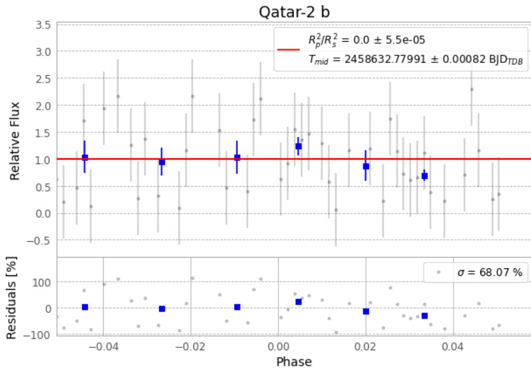
Figure 1 — FinalLightCurve_Qatar-2 b_2019-05-28.png (SHA-256 79c3b4c151e9b253...)
