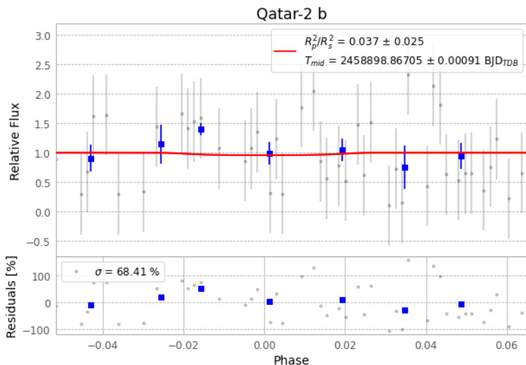
Figure 1 — FinalLightCurve_Qatar-2 b_2020-02-18.png (SHA-256 b8ae22b66b4ce73c...)
