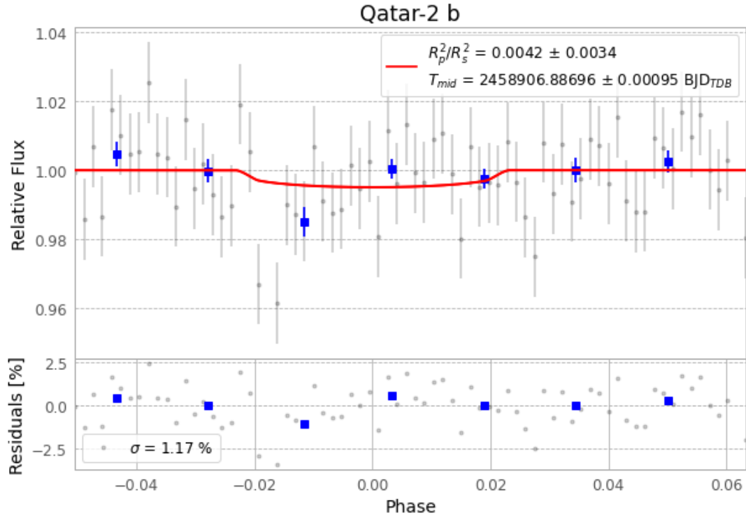
Figure 1 — FinalLightCurve_Qatar-2 b_2020-02-27.png (SHA-256 6e045680b497fc68...)
