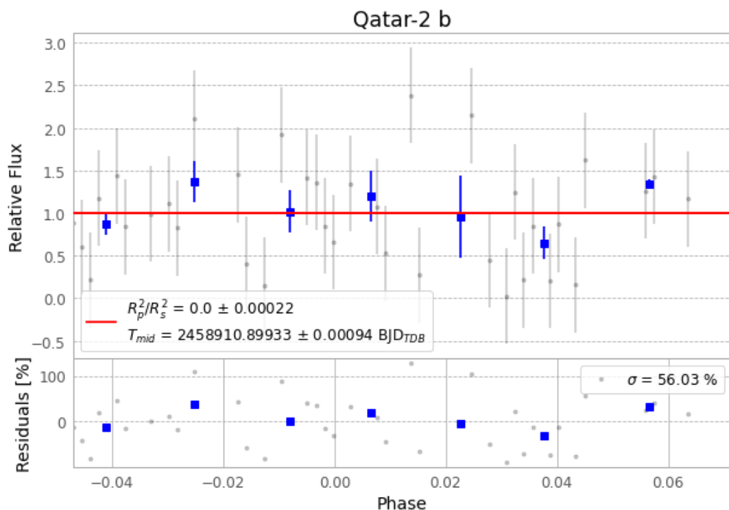
Figure 1 — FinalLightCurve_Qatar-2 b_2020-03-02.png (SHA-256 d8fa0458c678e1d7...)
