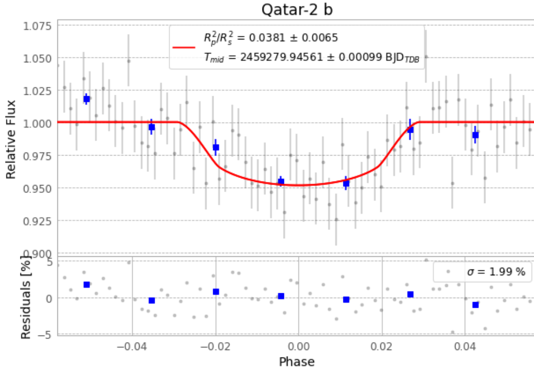
Figure 1 — FinalLightCurve_Qatar-2 b_2021-03-06.png (SHA-256 b418c308c777b04e...)
