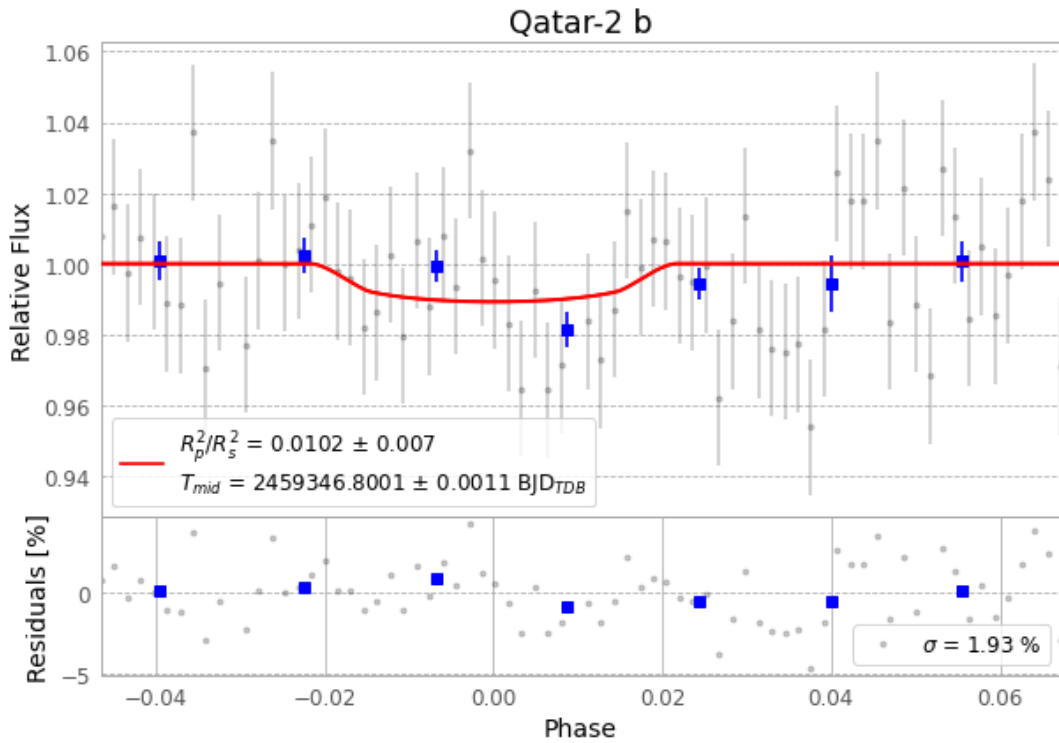
Figure 1 — FinalLightCurve_Qatar-2 b_2021-05-11.png (SHA-256 b0c91b56054b40bd...)
